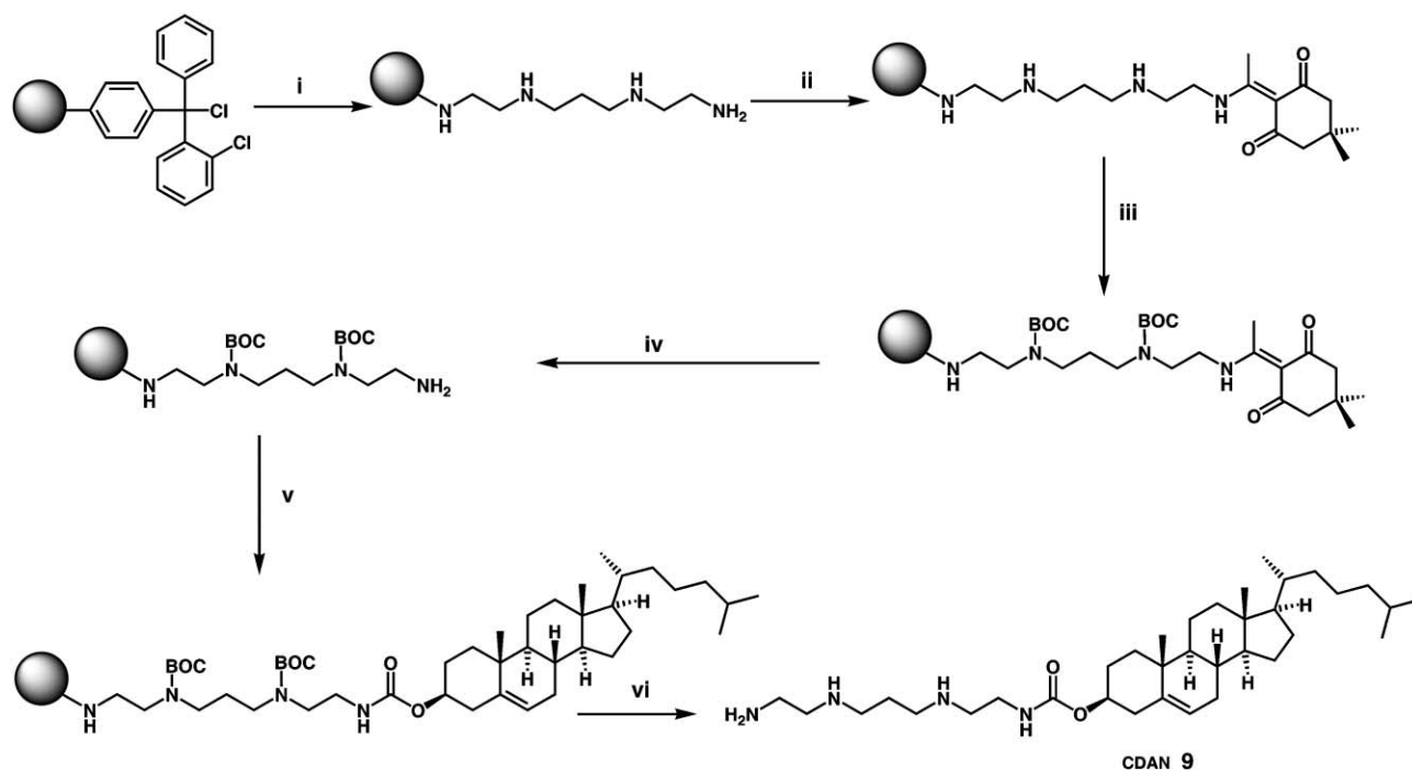
Scheme 1 Reagents and conditions: (i) polyamine (10 equiv.), \text{CH}_2\text{Cl}_2 , rt, 2 h, then MeOH (1000 equiv.), rt, 10 min; (ii) Dde-OH (10 equiv.), DMF, rt, 12 h; (iii) \text{Boc}_2\text{O} (5 equiv. per free amine), \text{NEt}_3 (2 equiv. per free amine), \text{CH}_2\text{Cl}_2 , rt, 4 h; (iv) 2% hydrazine hydrate in DMF, rt, 10 min (rpt step \times 2 ); (v) cholesterol chloroformate (10 equiv.), \text{NEt}_3 (3 equiv.), rt, 4 h; (vi) 50% TFA in \text{CH}_2\text{Cl}_2 , rt, 1 h, 93%. 40
