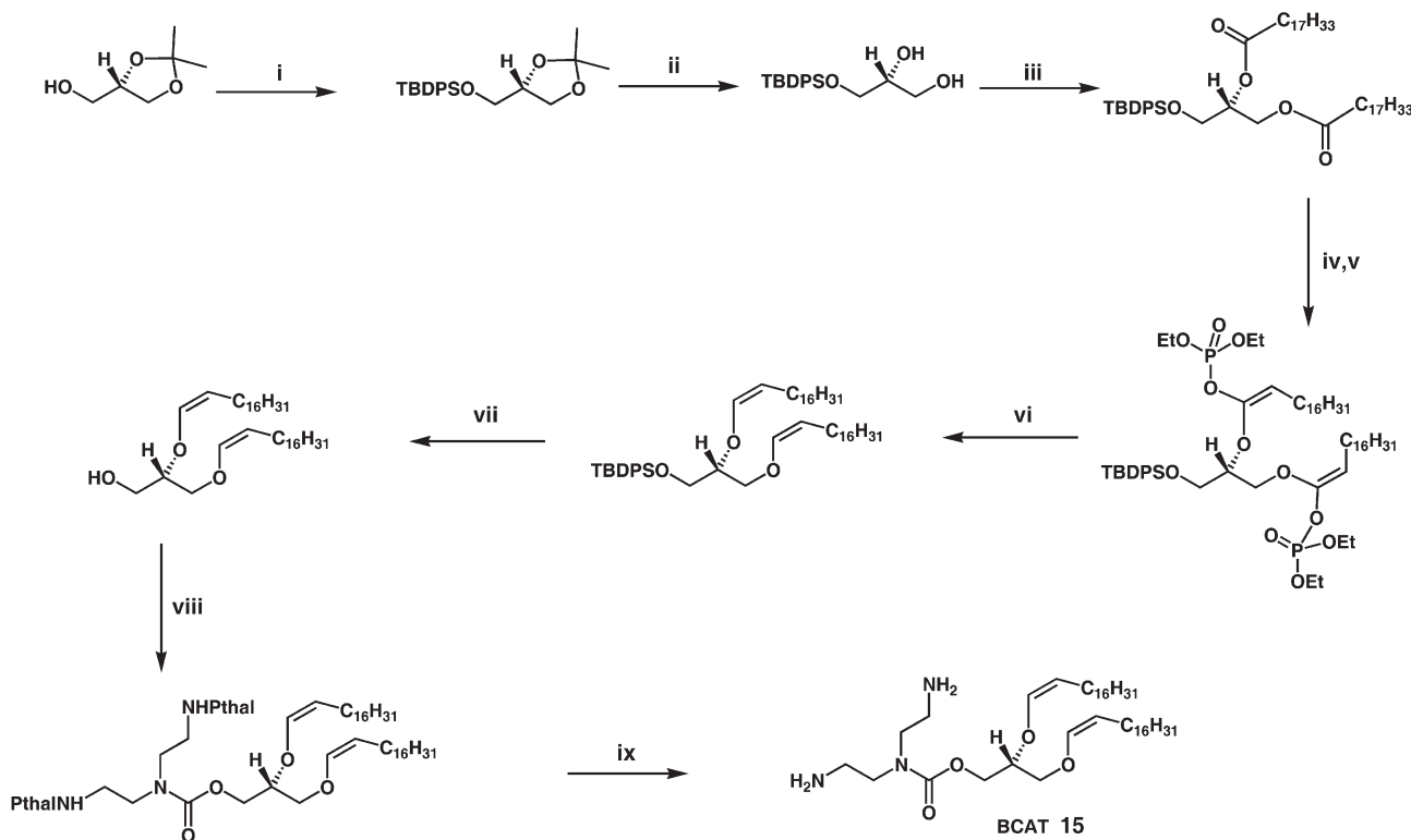
Scheme 4 Reagents and conditions: (i) TBDPS-Cl, imidazole; (ii) HCl, MeOH; (iii) oleoyl-Cl, pyridine; (iv) LDA; (v) \text{Et}_2\text{POCl} , HMPA; (vi) \text{Pd}(\text{PPh}_3)_4 , \text{Et}_3\text{Al} ; (vii) TBAF, TBAH; (viii) (a) \text{py}_2\text{CO} , \text{NEt}_3 (b) N,N' -diphthalamidylethylenetriamine; (ix) \text{N}_2\text{H}_4\text{--H}_2\text{O} . 49
