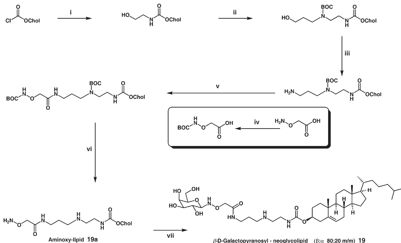
Scheme 5 Reagents and conditions: (i) \text{CH}_2\text{Cl}_2 , \text{HO}(\text{CH}_2)_2\text{NH}_2 (2.2 equiv.), 10 h, 97%; (ii) (a) \text{CH}_2\text{Cl}_2 , 0 °C, \text{NEt}_3 (3 equiv.), \text{MsCl} (2.5 equiv.), 10 min; then 1 h at rt, 98% (b) \text{THF} , \text{HO}(\text{CH}_2)_3\text{NH}_2 (10 equiv.), 6 h, 96% (c) \text{CH}_2\text{Cl}_2 , \text{NEt}_3 , \text{Boc}_2\text{O} , rt, 5 h, 90%; (iii) (a) \text{CH}_2\text{Cl}_2 , 0 °C, \text{NEt}_3 (3 equiv.), \text{MsCl} (2.5 equiv.), 10 min; then 2 h at rt, 90% (b) \text{DMF} , 80 °C, \text{NaN}_3 (5 equiv.), \text{NaI} (1 equiv.), 3 h, 95% (c) \text{THF} , \text{PMe}_3 (1.15 equiv.), rt, 3 h (d) \text{H}_2\text{O}/\text{NH}_3 , 88%; (iv) \text{CH}_2\text{Cl}_2 , \text{NEt}_3 , \text{Boc}_2\text{O} , rt, 5 h, 98%; (v) (a) \text{EtOAc} , \text{NHS} (1 equiv.), \text{DCC} (1 equiv.), 10 h, rt (b), \text{EtOAc}/\text{THF} 95/5 v/v, \text{NEt}_3 (pH8), 2 h, rt, 90%; (vi) \text{CH}_2\text{Cl}_2 , \text{TFA} (15 equiv.), 0 °C, \text{N}_2 , 5 h, 86%; (vii) saccharide, \text{AcOH}/\text{DMF} 1/1 v/v, rt. 98
